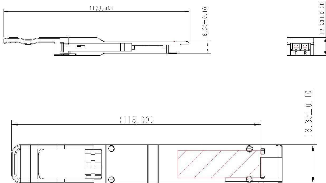
Figure 3. Mechanical Dimensions
