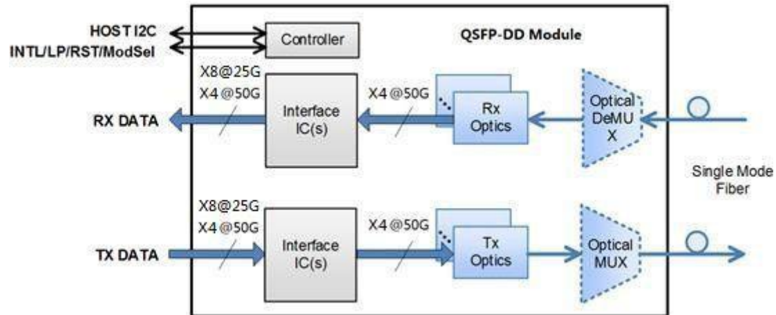
Figure 1. Transceiver Block Diagram
