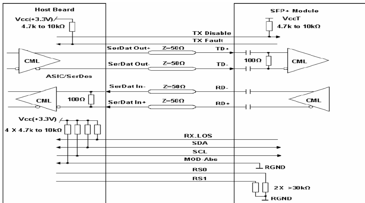
Recommended High-speed Interface Circuit
