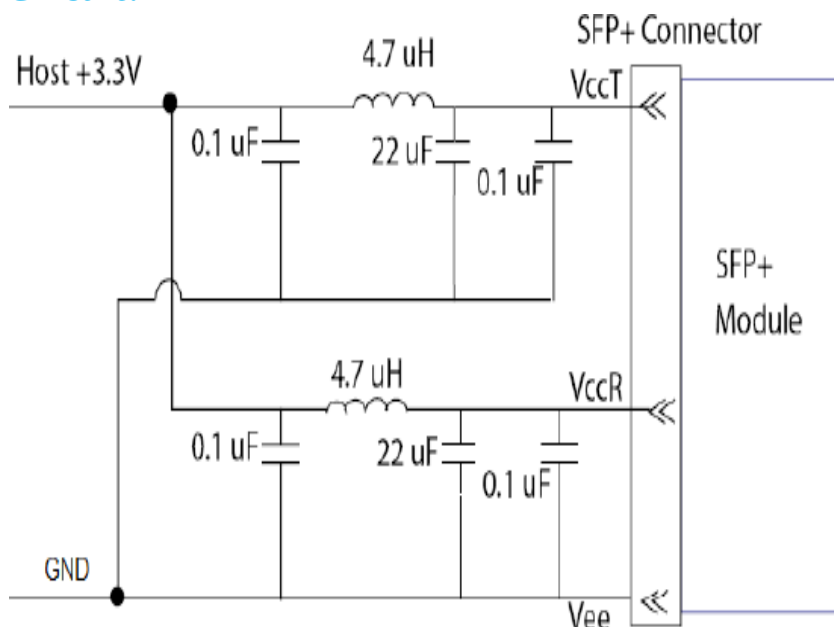
Recommended Host Board Power Supply Circuit
