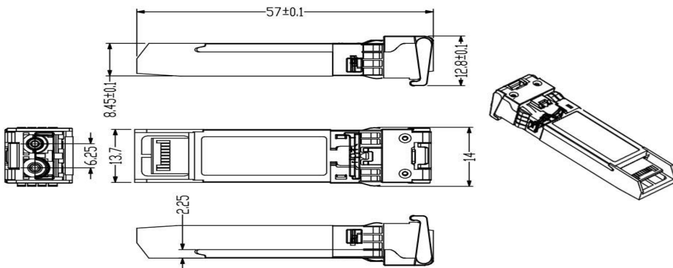
Mechanical Drawing
