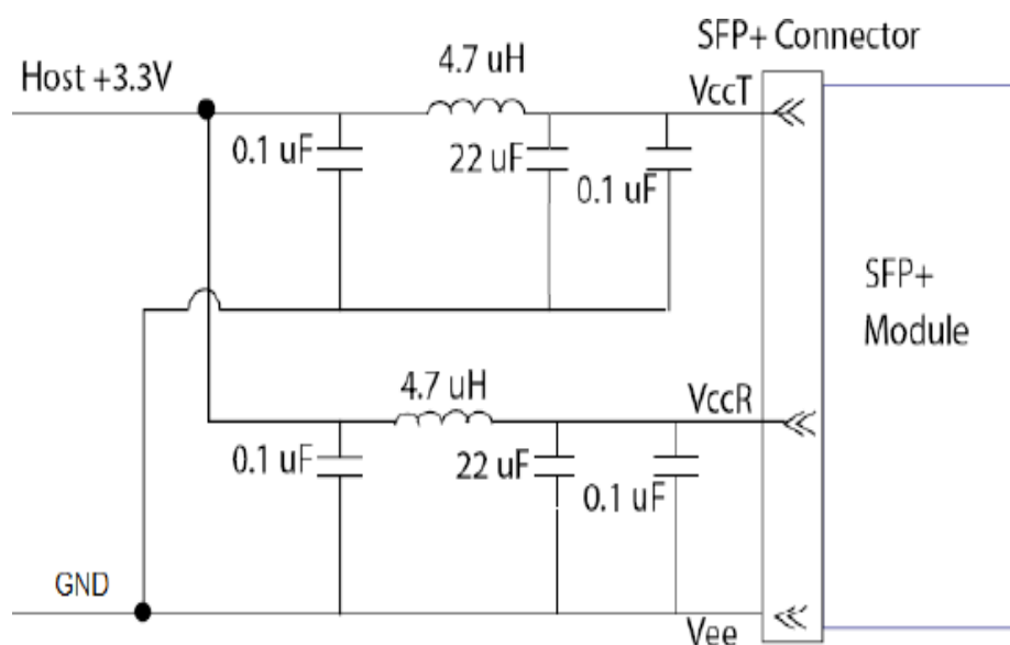
Recommended Host Board Power Supply Circuit
