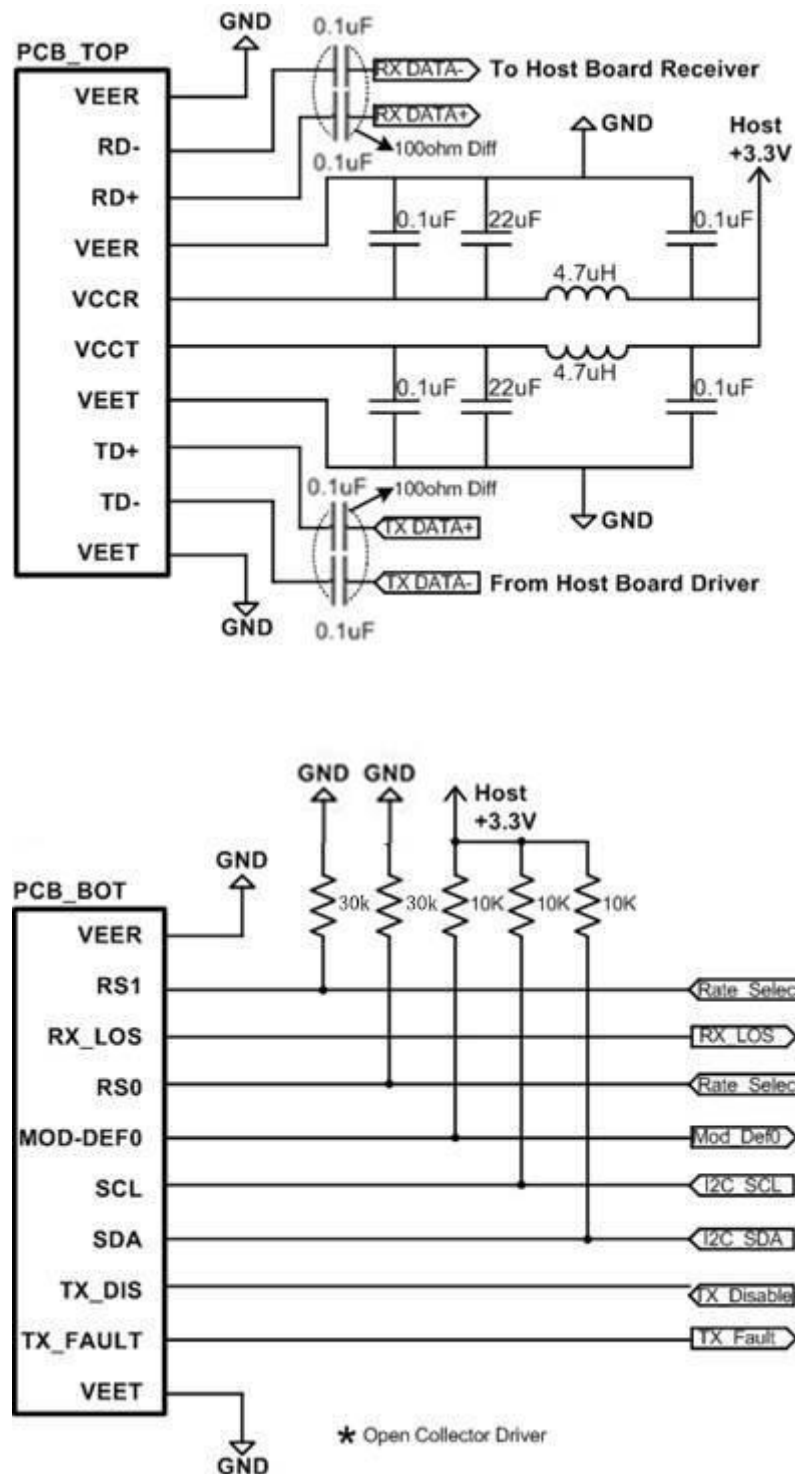
Recommended High-speed Interface Circuit
