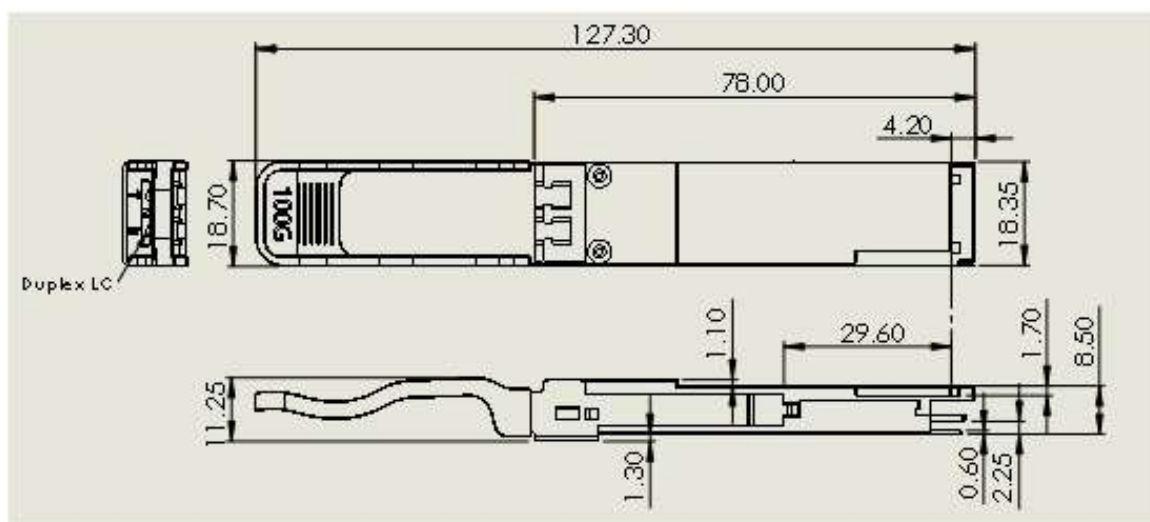
Figure 5. Mechanical Outline
