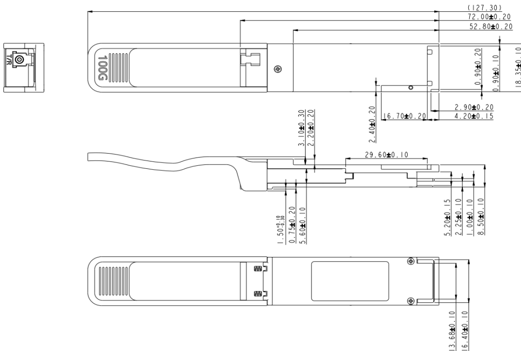
Figure3 100G LR1 BIDI QSFP28 Mechanical Dimensions
