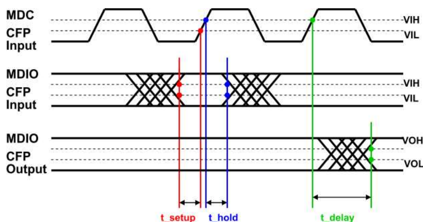
Figure 4. 100Gb/s CFP MDIO &amp; MDC Timing Diagram
