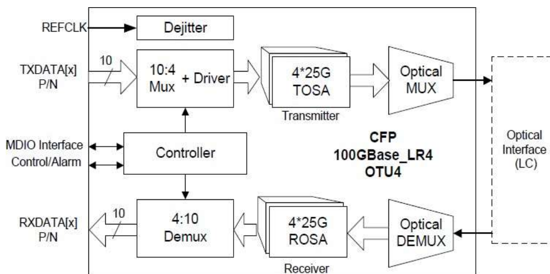
Figure 5. 10km 100Gb/s CFP internal structure
